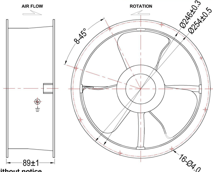
Dimensions Drawing
