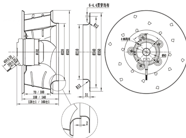
Dimensions Drawing
