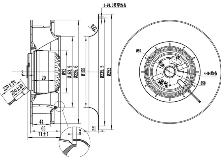
Dimensions Drawing
