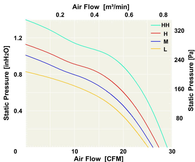
Air Flow & Static Pressure Curve
