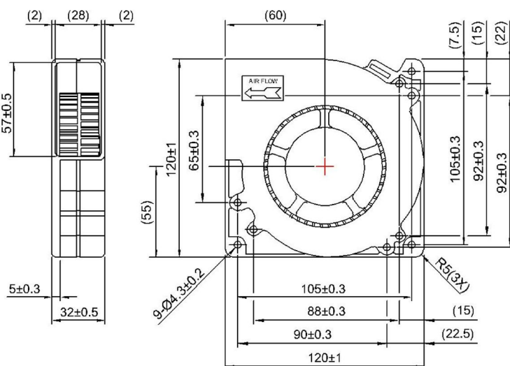
Dimensions Drawing
