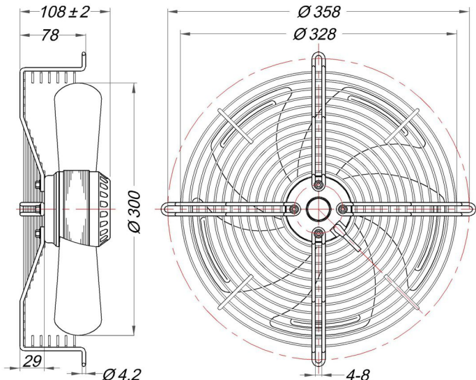
Dimensions Drawing
