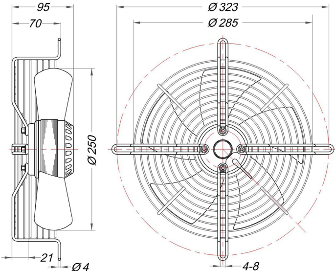
Dimensions Drawing
