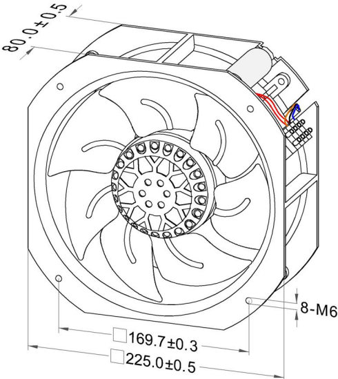
Dimensions Drawing
