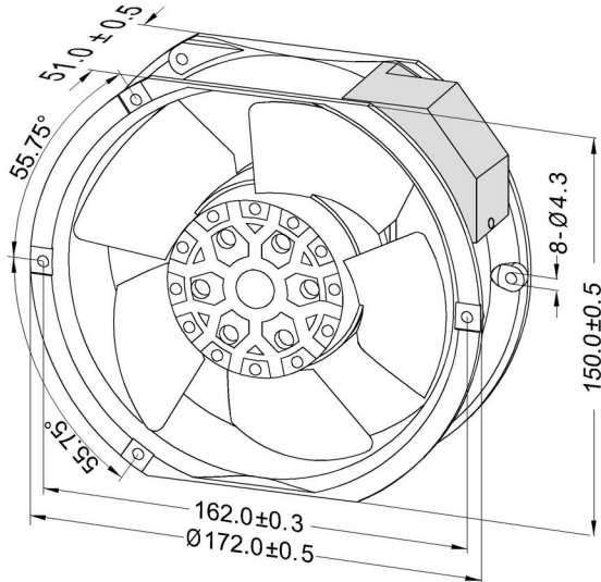
Dimensions Drawing
