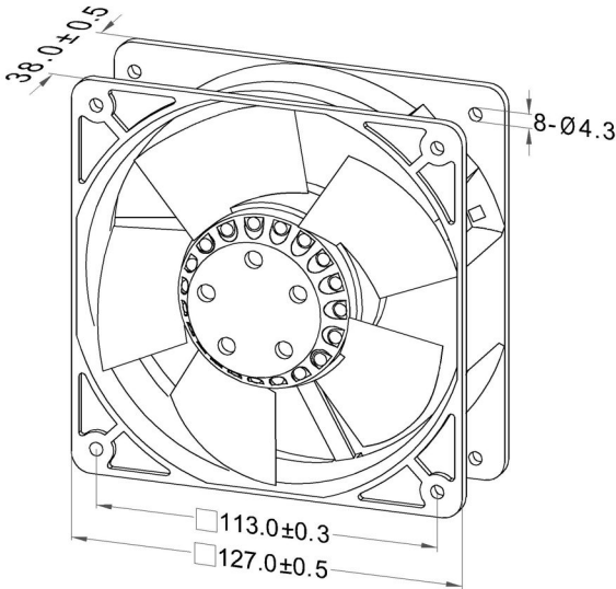
Dimensions Drawing
