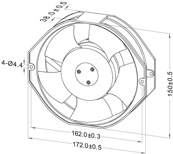
Dimensions Drawing
