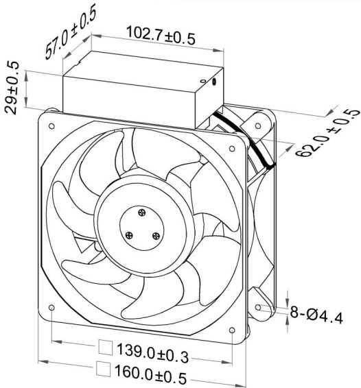
Dimensions Drawing
