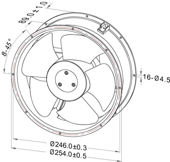
Dimensions Drawing
