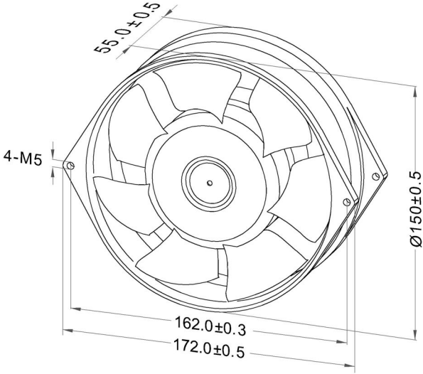
Dimensions Drawing
