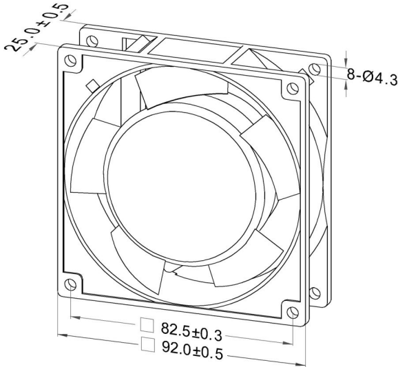
Dimensions Drawing
