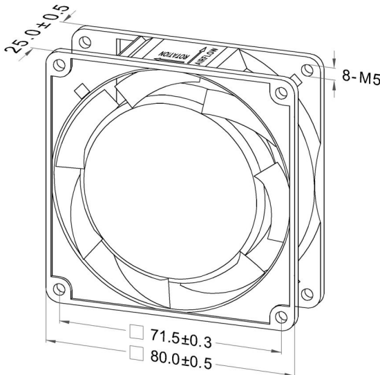
Dimensions Drawing
