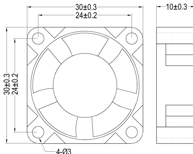
Dimensions Drawing
