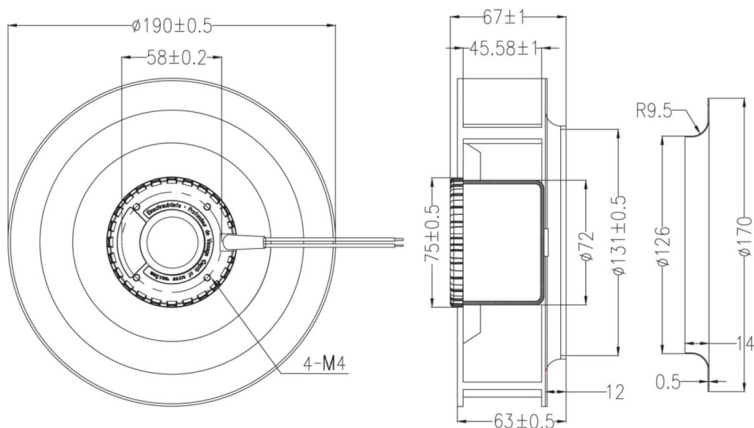
Dimensions Drawing
