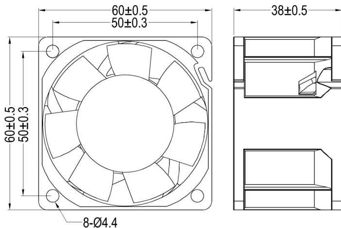
Dimensions Drawing
