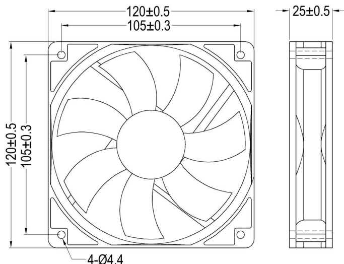
Dimensions Drawing
