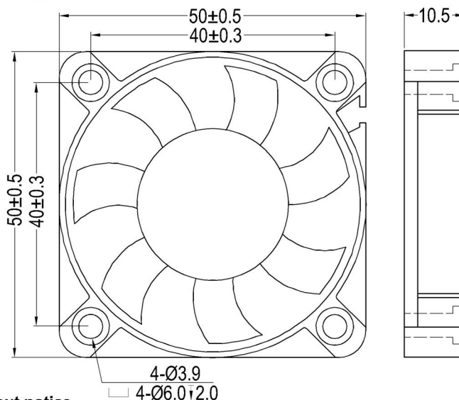
Dimensions Drawing
